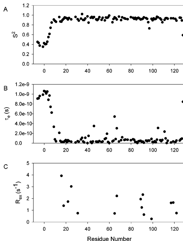
FIGURE 4: Model Free analysis of backbone NMR relaxation data for 15.5K free in solution at 20 °C. Data recorded at 500 and 600 MHz ( ^1\text{H} ) were used to fit (a) S^2 , (b) \tau_e , and (c) R_{\text{ex}} for \tau_m = 11.75 \text{ ns} as described in Experimental Procedures.
